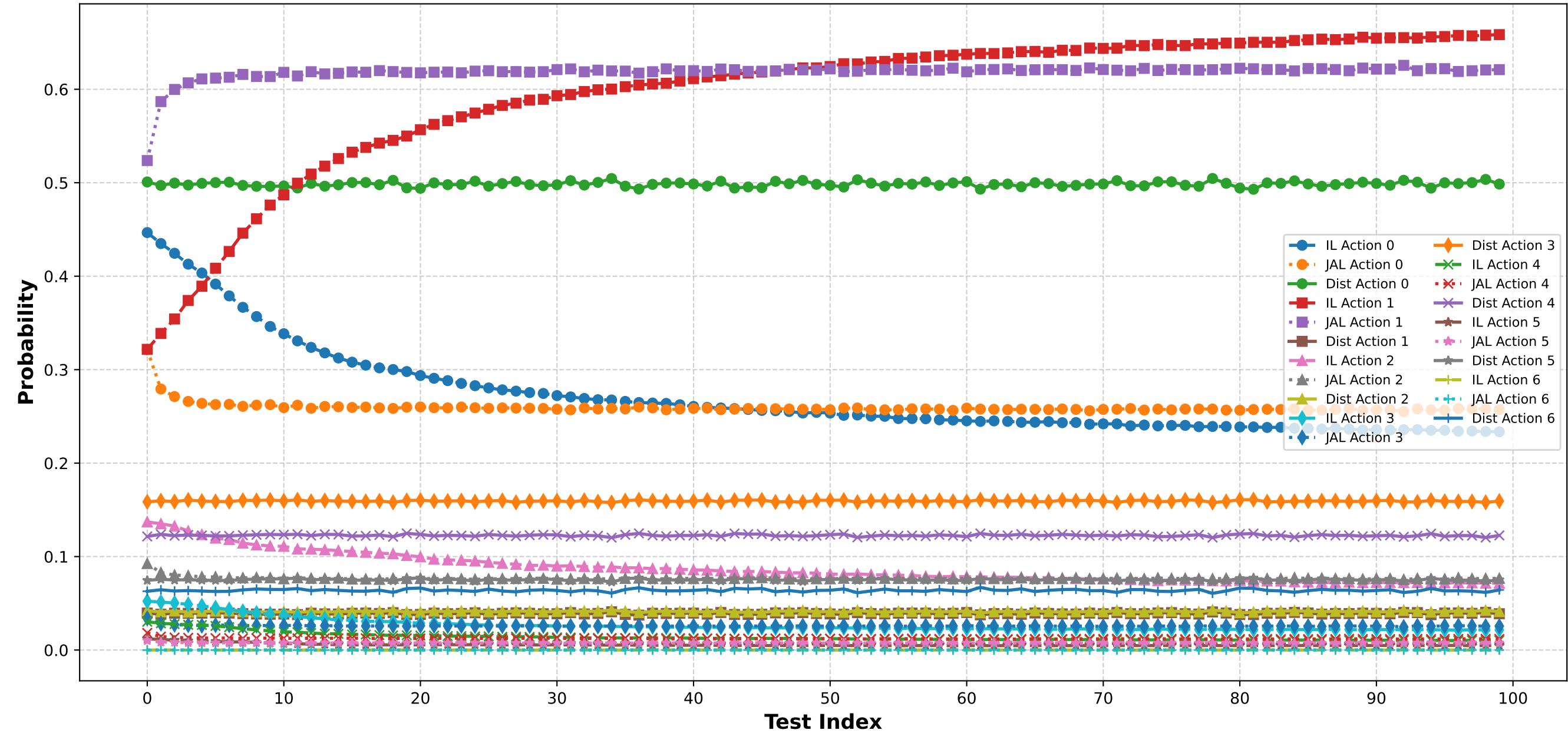
Action Probability Evolution Comparison
